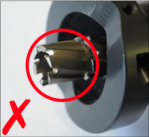
INCORRECT. Installed cutters should NOT remain protruding from the cutter assembly. Ensure that cutters are fully retracted inside the cutter assembly before using the Drill Jig.
