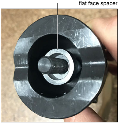
The flat face spacer is used with square pipe ONLY
