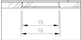
Flat face (square) rail applications require the flat face spacer installed in the Drill Jig.
