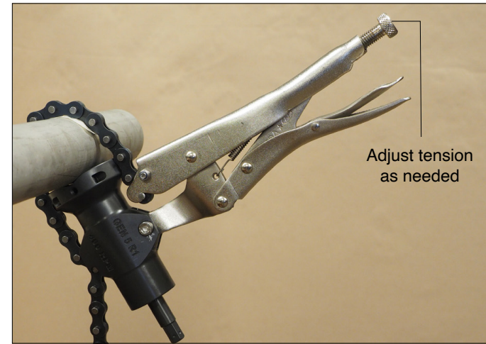
Adjust tension to ensure the clamp body is secure on the rail.
