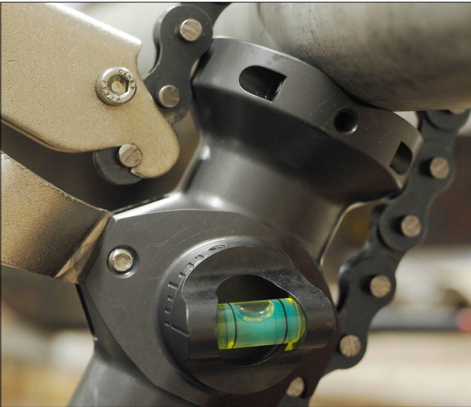
Above: The drill Jig's level bubble should be centered before the drilling to enable consistent angle drilling at your set angle.
