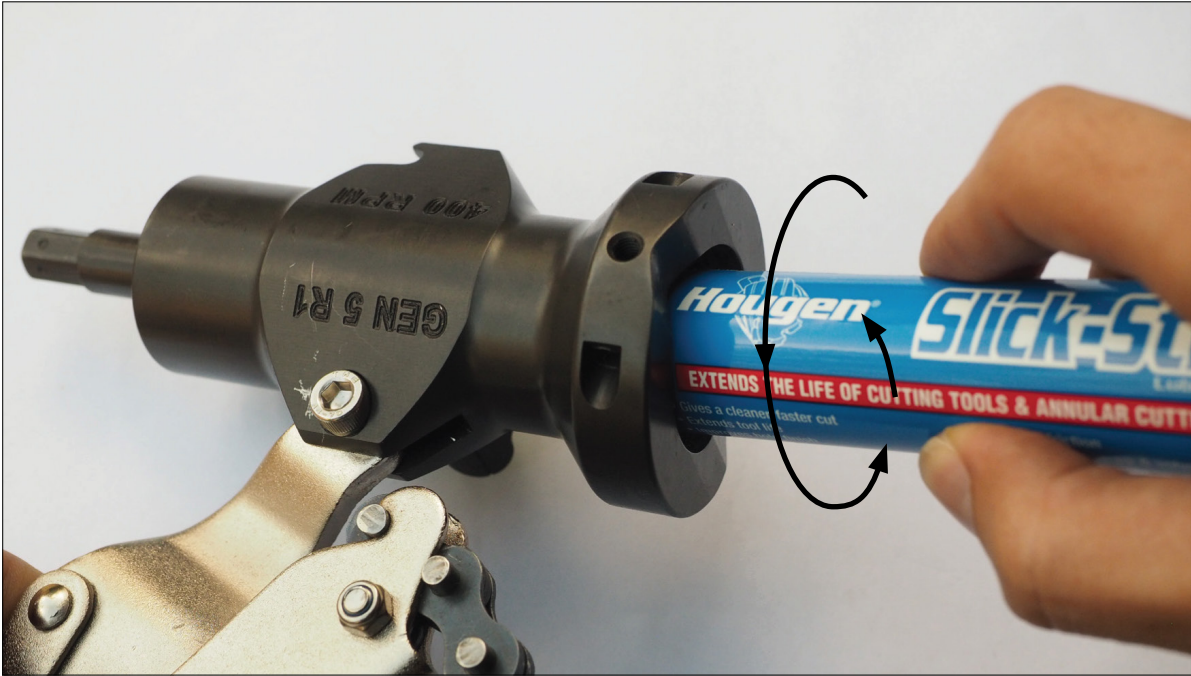
5.1 IMPORTANT! Lubricate the cutters before drilling each hole. A light twist action will supply a sufficient amount.
