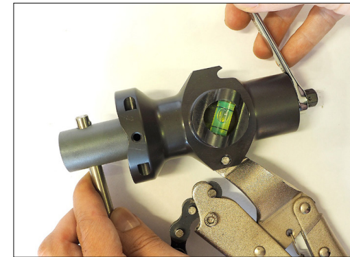
Fig. 3.4 Use the cutter removal tool and wrench provided to remove or secure the cutters. Note the cutter removal tool's 15mm side (shallow) and 16mm side (deep).
