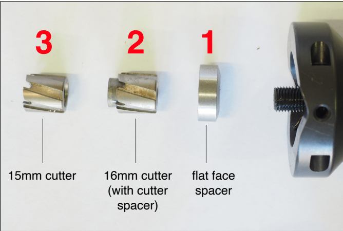
The flat face spacer is installed FIRST, followed by the cutter installation (see step 3). Remember to fully extend the cutter end of the Drill Jig (as shown).
