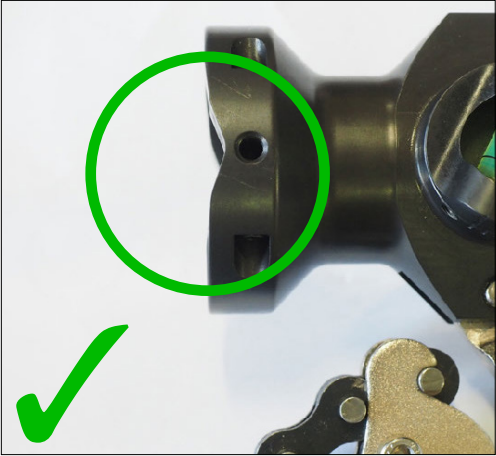
CORRECT. Cutters are installed and fully retracted inside the cutter assembly.
