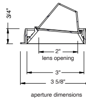
aperture dimensions
