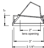
aperture dimensions
