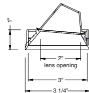
aperture dimensions
