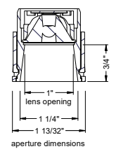
ceiling cutout 1-7/16" square ceiling thickness 1/8" to 1 1/2"
