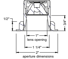
ceiling cutout 1-3/4" square ceiling thickness 1/8" to 1 1/2"
