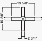
TR-X1 : X Connector - one side/ feed in, three sides/feed out
