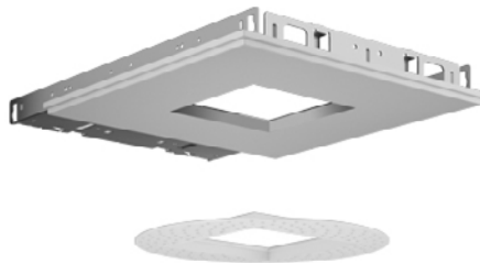
1. Fasten mud frame to ceiling.
